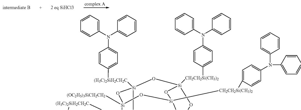
<Reaction Scheme 2>
